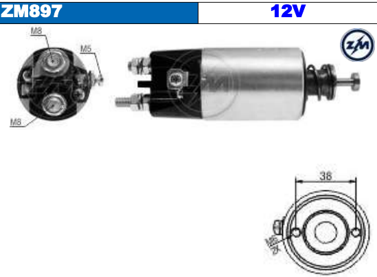
MITSUBISHI: M371XB0271
